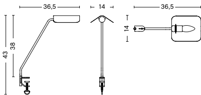
APEX DESK CLIP LAMP Width 14 cm Depth 36,5 cm Height 43 cm Weight 0,66 kg Max. table/shelf thickness 4 cm
