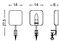
APEX CLIP LAMP Width 14 cm Depth 8 cm Height 27,5 cm Weight 0,57 kg Max. table/shelf thickness 4 cm
