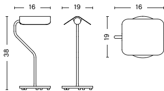
APEX TABLE LAMP Width 19 cm Depth 16 cm Height 38 cm Weight 1,56 kg
