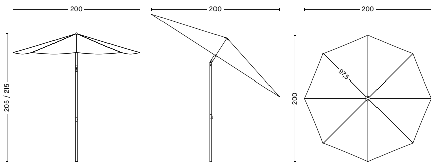
TERRAZZA PARASOL | OCTAGON Diameter 200 cm Height 205 / 215 cm Tilt angle 30° Pole diameter 3,63 cm Weight 2,8 kg
