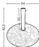
TERRAZZA PARASOL BASE Diameter 54 cm Height 42,5 cm Pole diameter 4,2 cm Weight 35 kg
