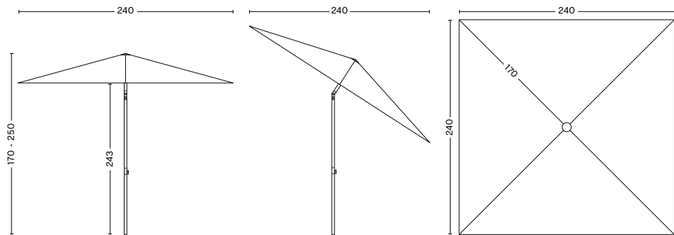
TERRAZZA PARASOL | SQUARE Width 240 cm Length 240 cm Minimum height 170 cm Maximum height 250 cm Tilt angle 30° Pole diameter 3,52 cm Weight 5,3 kg
