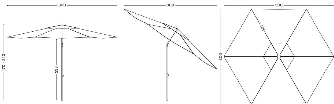
TERRAZZA PARASOL | HEXAGON Diameter 300 cm Minimum height 170 cm Maximum height 240 cm Tilt angle 30° Pole diameter 3,52 cm Weight 5,8 kg
